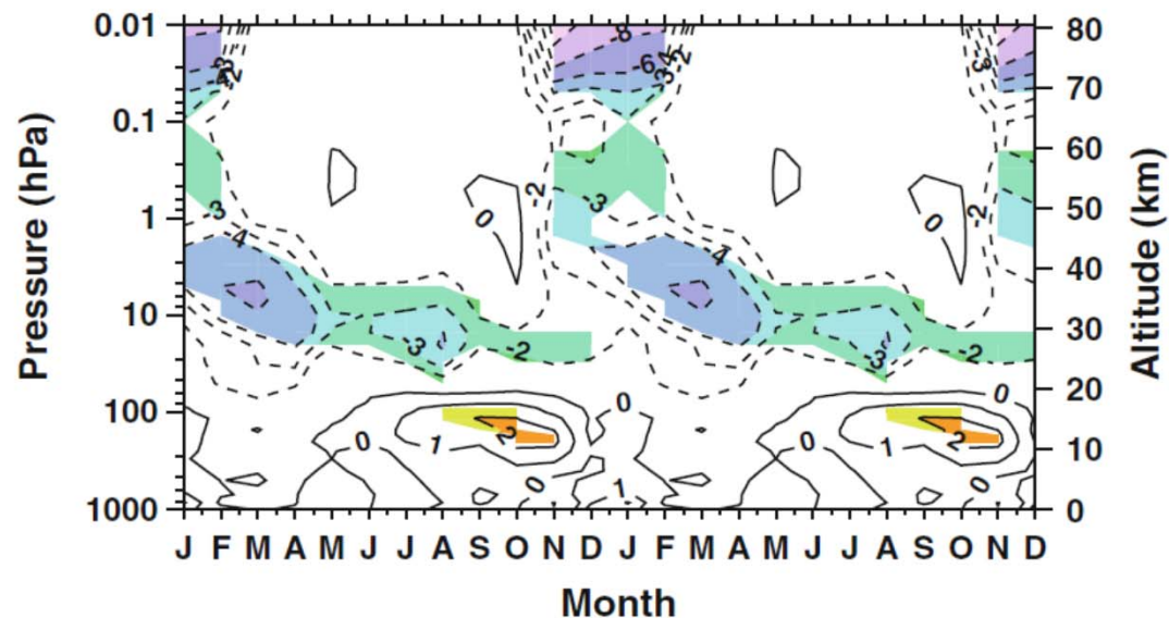
Fig. 8 Monthly mean response of zonal mean O 3 , (%) to GCR, SPE, and EEP averaged over 60°–90°N. The contours are plotted for: –12.0, –10.0, –8.0, –6.0, –4.0, –3.0, –2.0, 0.0, 1.0, 2.0, and 3.0 %. Results are averaged from 1960 to 2005. Solid contours indicate positive, dotted contours negative changes. Color pattern indicates the regions where the changes are judged statistically significant at or better than 10 % level. Twelve months of the monthly run climatology are repeated
